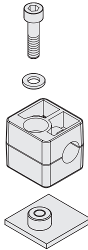
DCK-S-1-SRC-WA-PL (Grupa 1)
